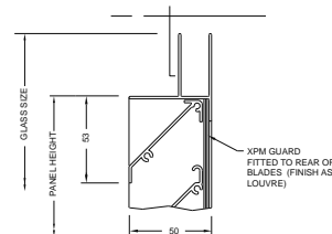
590. STANDARD HEAD DETAIL
