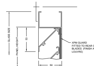
600. STANDARD HEAD DETAIL
