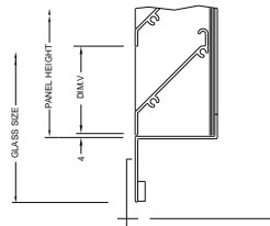
606. 50 BLADE CILL DETAIL
