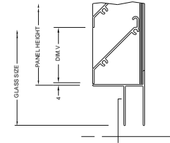
591. 50 BLADE CILL DETAIL
