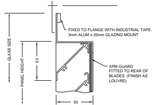
605. STANDARD HEAD DETAIL
