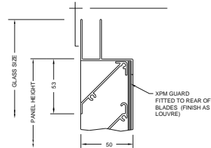
595. STANDARD HEAD DETAIL
