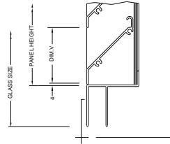
596. 50 BLADE CILL DETAIL
